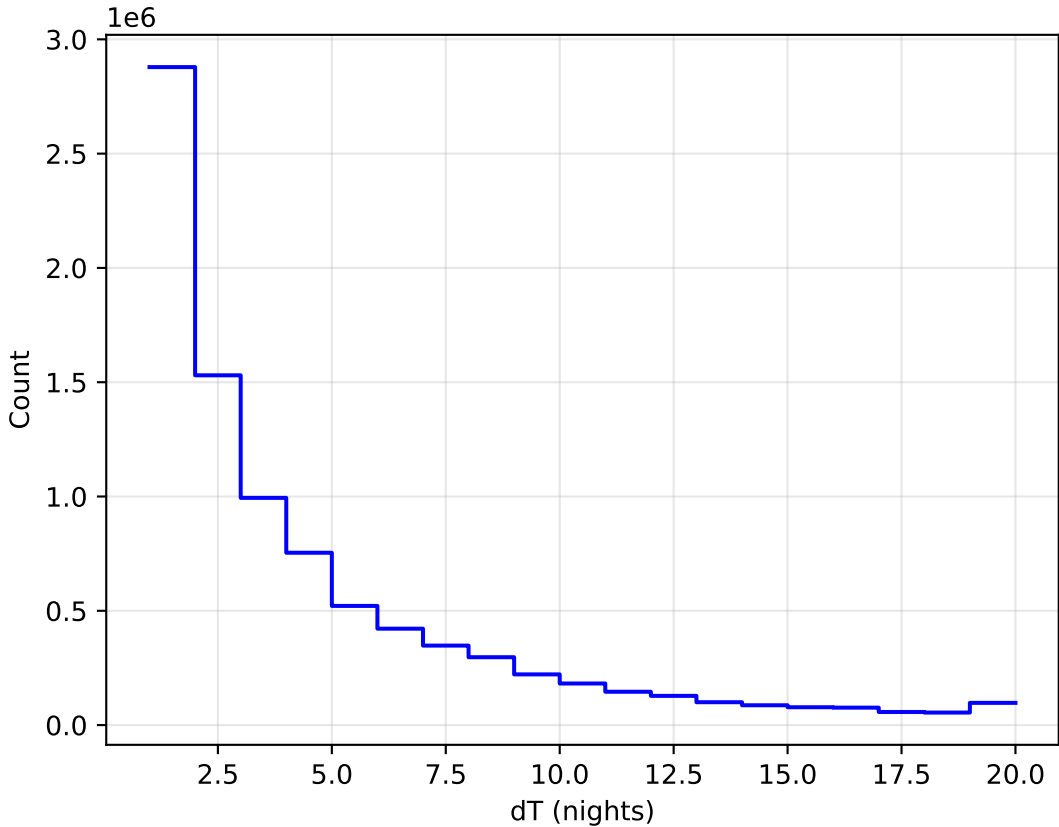
internal_u_expt30_nscale1.1v3.4_10yrs All sky all bands: DeltaNight Histogram
