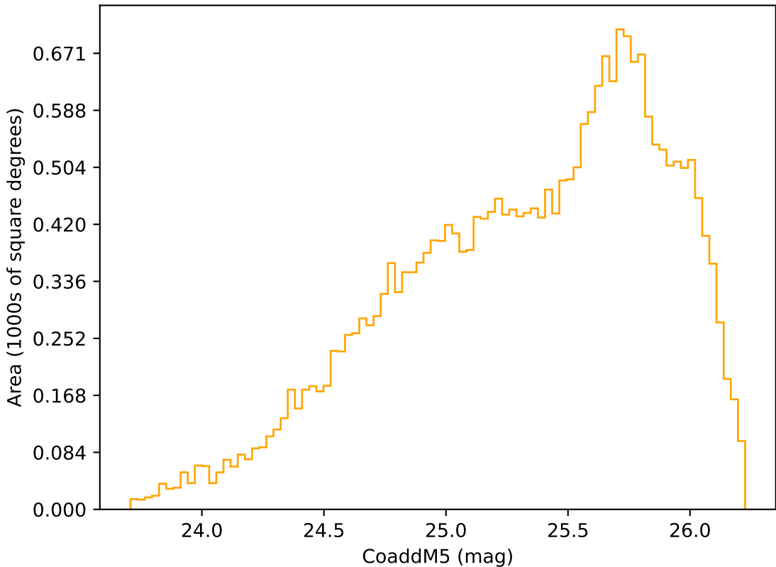
internal_u_expt30_nscale1.1v3.4_10yrs Yr 3-4 r band: CoaddM5
