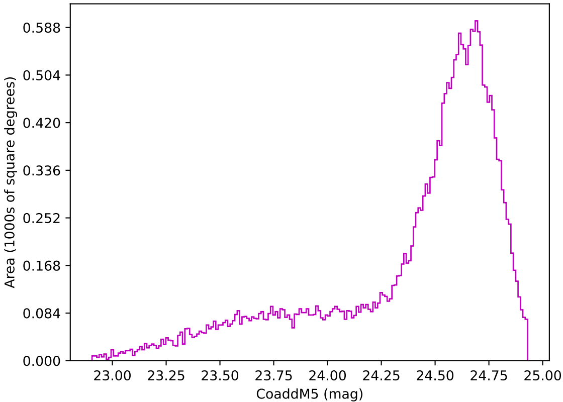
internal_u_expt30_nscale1.1v3.4_10yrs Yr 1 z band: CoaddM5
