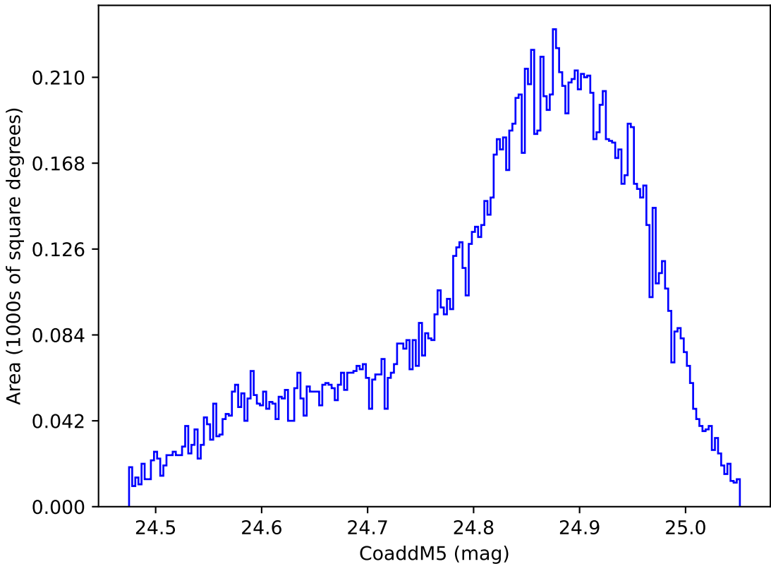
internal_u_expt30_nscale1.1v3.4_10yrs WFD y band: CoaddM5
