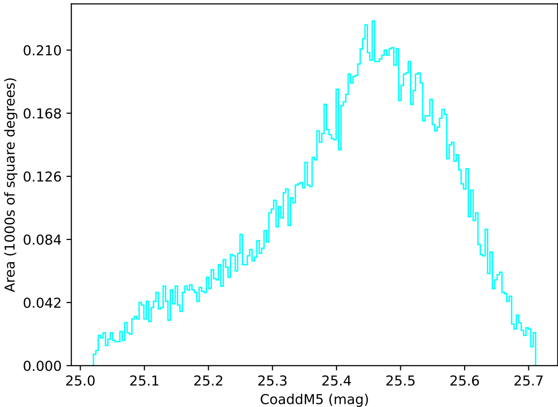
internal_u_expt30_nscale1.1v3.4_10yrs WFD u band: CoaddM5
