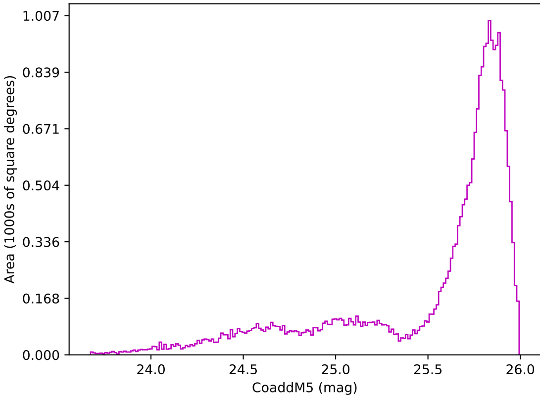
internal_u_expt30_nscale1.1v3.4_10yrs All sky z band: CoaddM5
