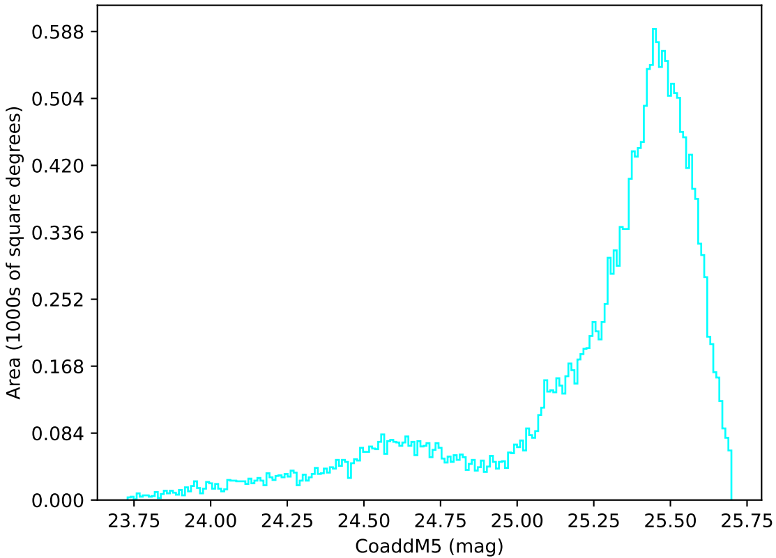
internal_u_expt30_nscale1.1v3.4_10yrs All sky u band: CoaddM5
