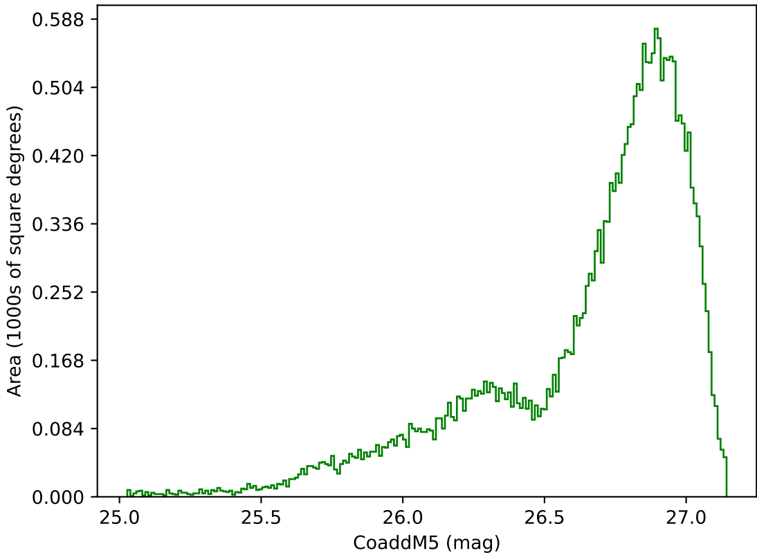
internal_u_expt30_nscale1.1v3.4_10yrs All sky g band: CoaddM5
