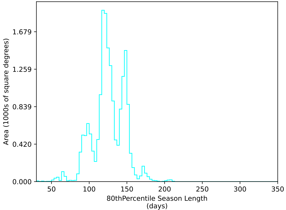
internal_u_expt30_nscale1.1v3.4_10yrs WFD u band: 80thPercentile Season Length
