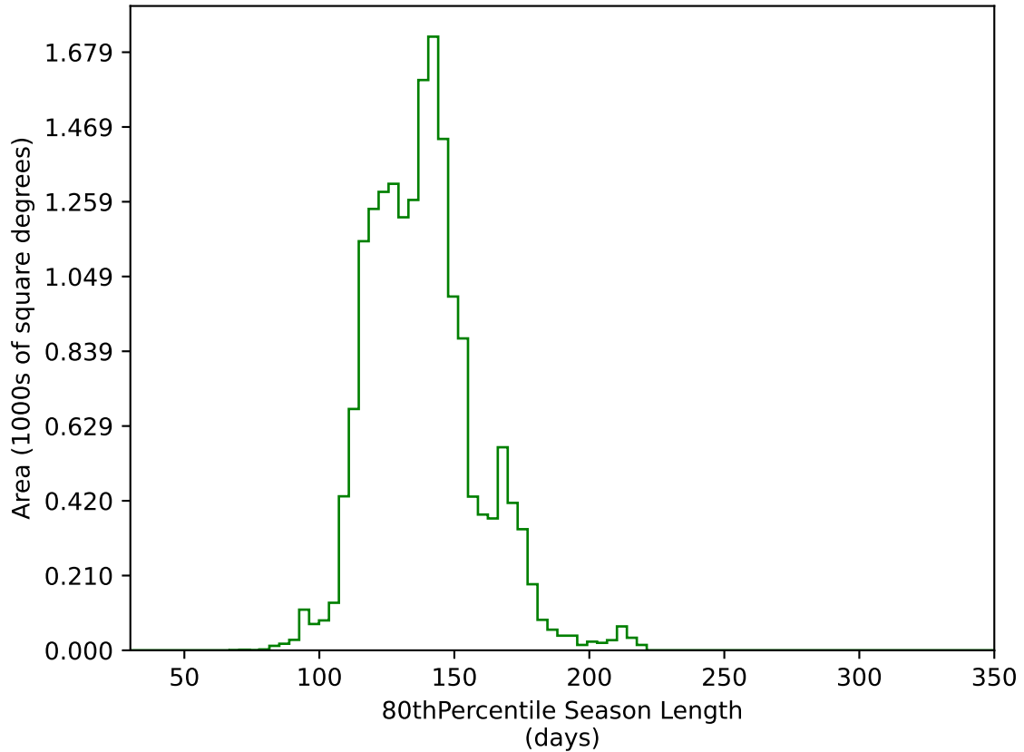
internal_u_expt30_nscale1.1v3.4_10yrs WFD g band: 80thPercentile Season Length
