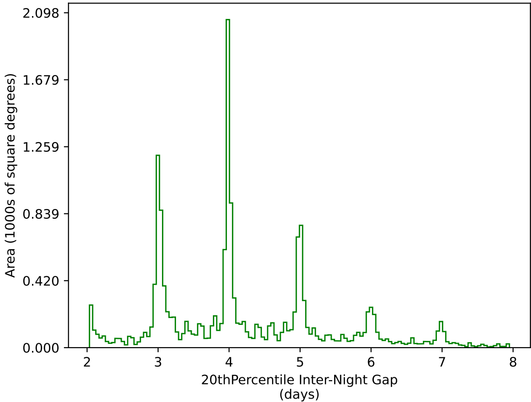
internal_u_expt30_nscale1.1v3.4_10yrs WFD g band: 20thPercentile Inter-Night Gap
