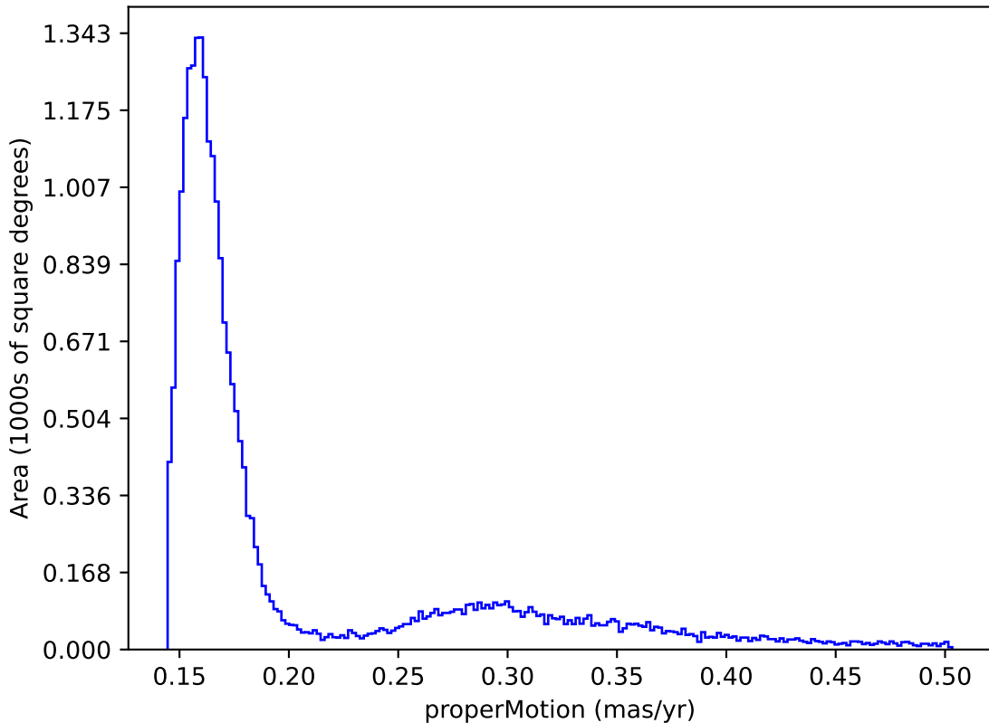
internal_u_expt30_nscale1.1v3.4_10yrs : properMotion
