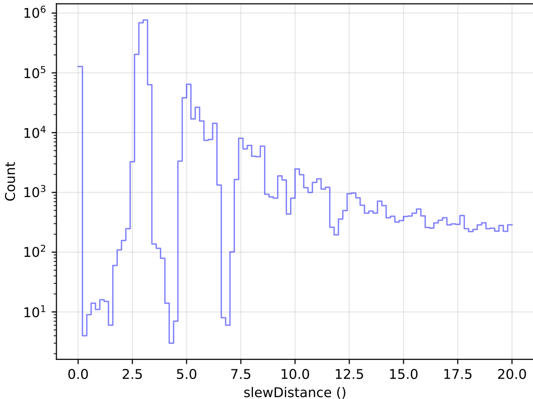
internal_u_expt30_nscale1.1v3.4_10yrs All visits: Zoom Slew Distance Histogram
