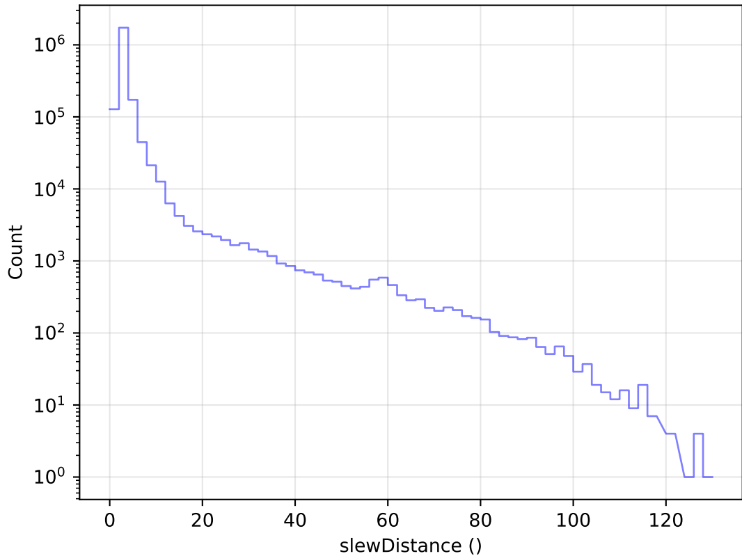
internal_u_expt30_nscale1.1v3.4_10yrs All visits: Slew Distance Histogram
