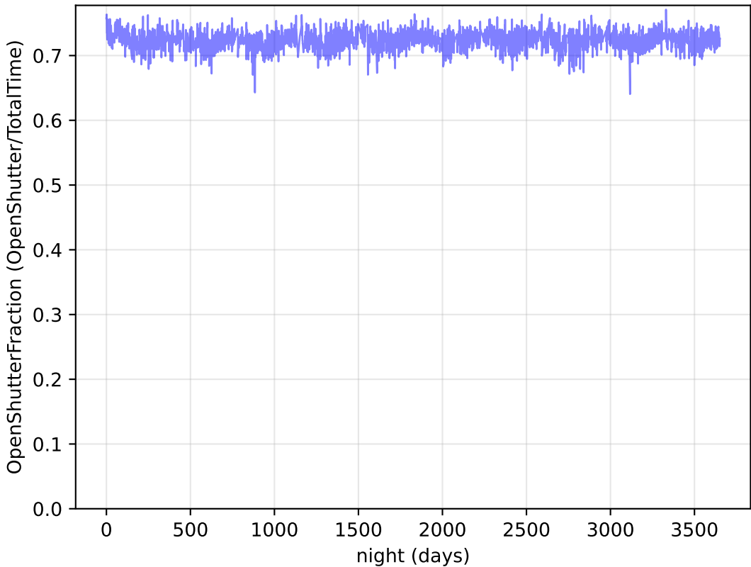
internal_u_expt30_nscale1.1v3.4_10yrs : OpenShutterFraction
