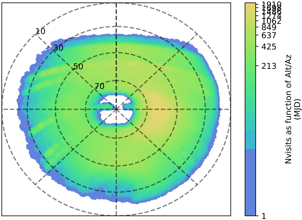
internal_u_expt30_nscale1.1v3.4_10yrs y: Nvisits as function of Alt/Az
