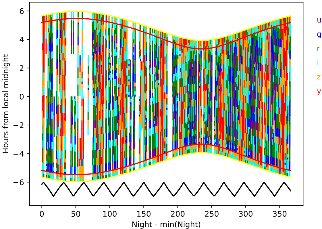
internal_u_expt30_nscale1.1v3.4_10yrs year 9-10: Hourglass
