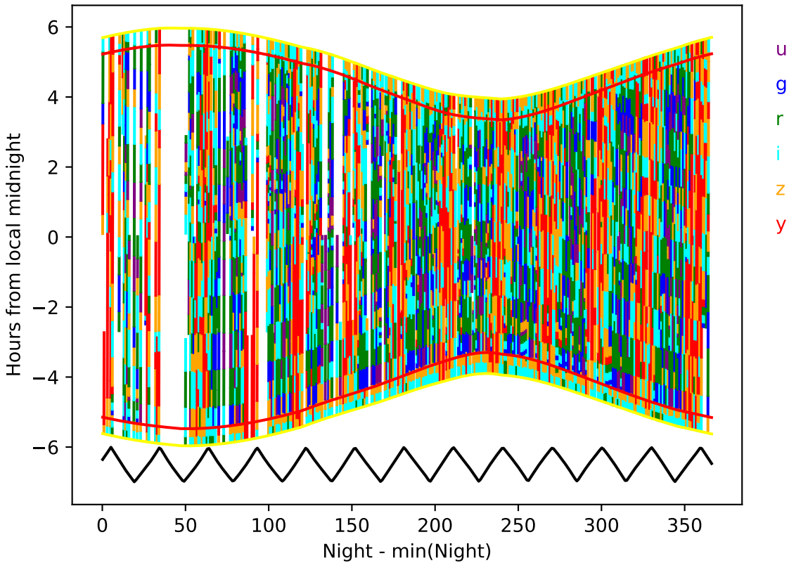
internal_u_expt30_nscale1.1v3.4_10yrs year 6-7: Hourglass
