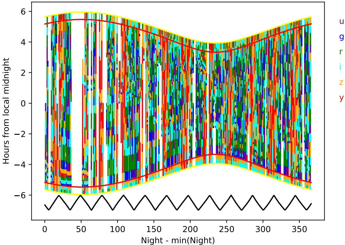
internal_u_expt30_nscale1.1v3.4_10yrs year 2-3: Hourglass
