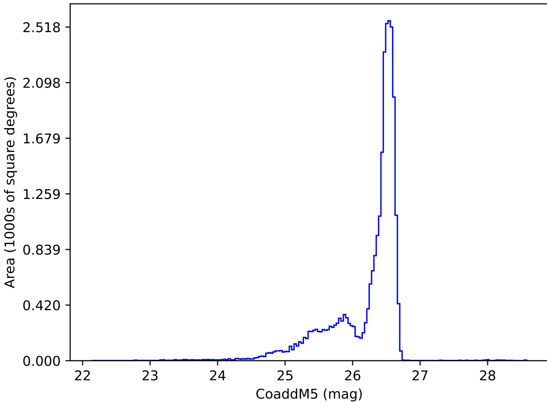
internal_u_expt30_nscale1.1v3.4_10yrs i: CoaddM5
