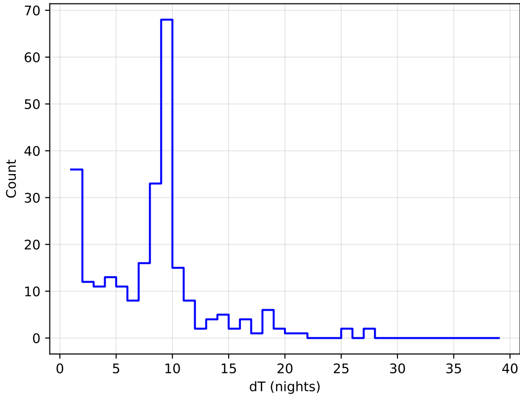
internal_u_expt30_nscale1.1v3.4_10yrs all bands: DD:ELAISS1 Delta Nights Histogram
