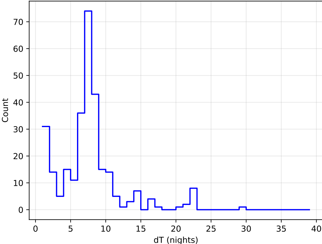
internal_u_expt30_nscale1.1v3.4_10yrs all bands: DD:EDFS Delta Nights Histogram
