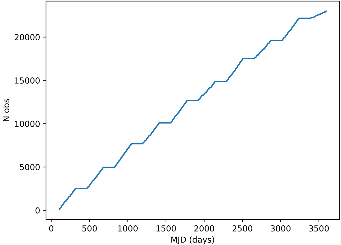
internal_u_expt30_nscale1.1v3.4_10yrs all bands: DD:EDFS Cumulative NVisits
