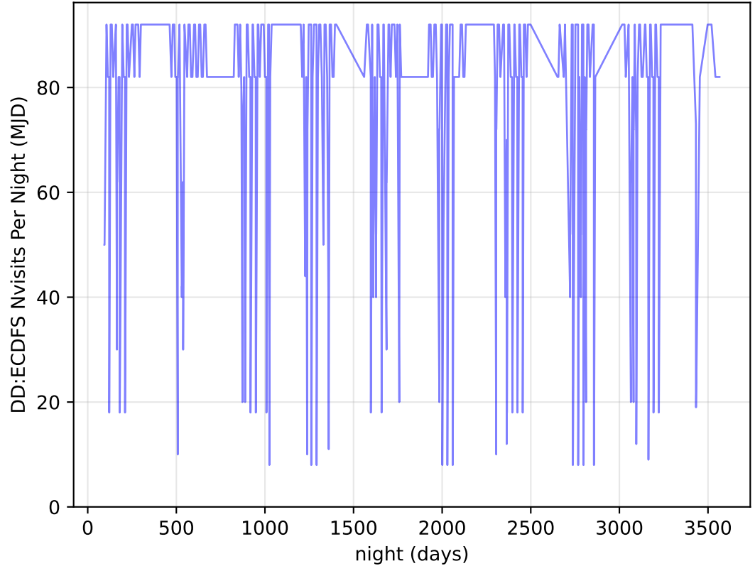
internal_u_expt30_nscale1.1v3.4_10yrs all bands: DD:ECDFS Nvisits Per Night
