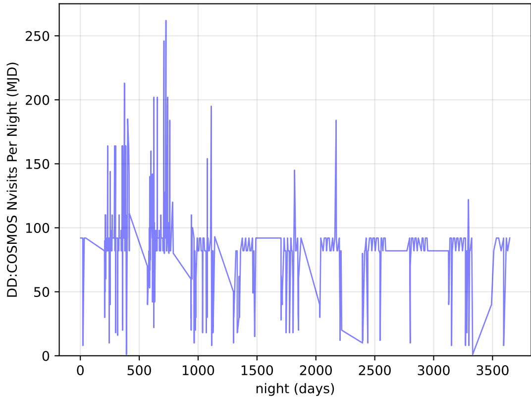
internal_u_expt30_nscale1.1v3.4_10yrs all bands: DD: COSMOS Nvisits Per Night
