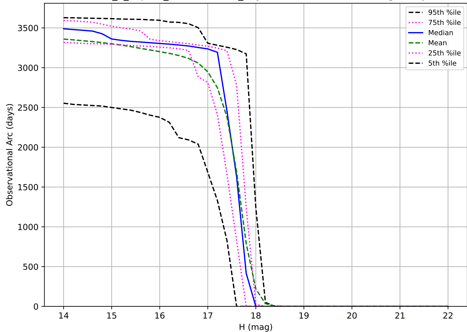
internal_u_expt30_nscale1.0v3.4_10yrs: Observational Arc Length Trojan
