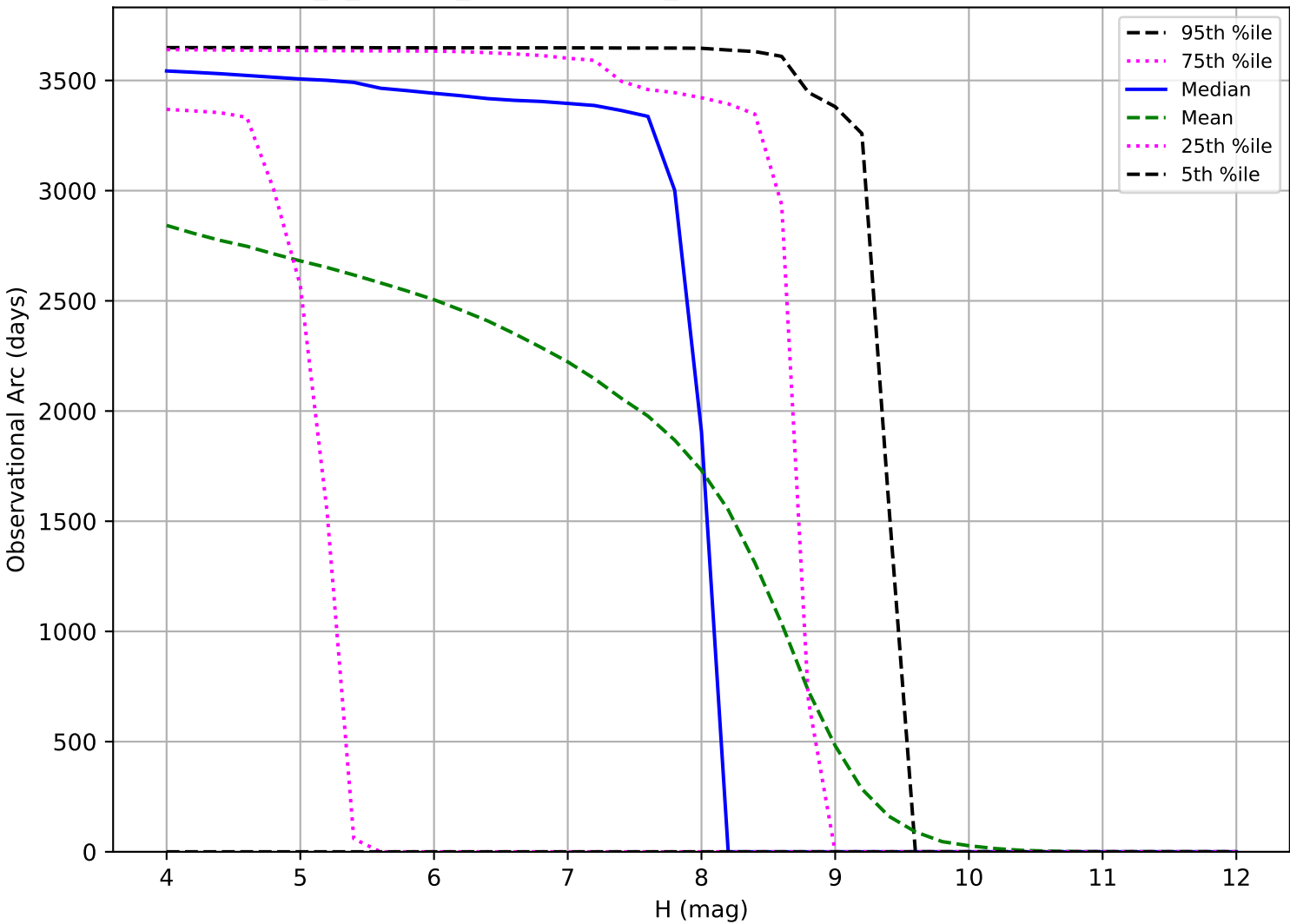
internal_u_expt30_nscale1.0v3.4_10yrs: Observational Arc Length TNO
