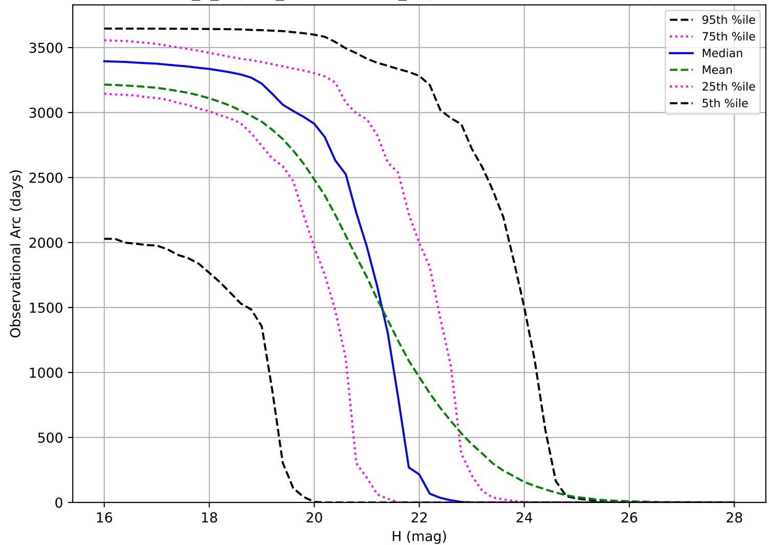
internal_u_expt30_nscale1.0v3.4_10yrs: Observational Arc Length PHA
