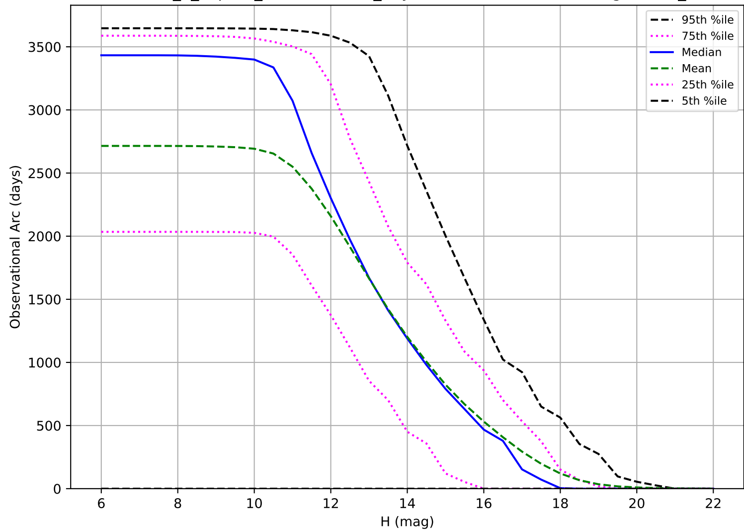
internal_u_expt30_nscale1.0v3.4_10yrs: Observational Arc Length OCC_r5
