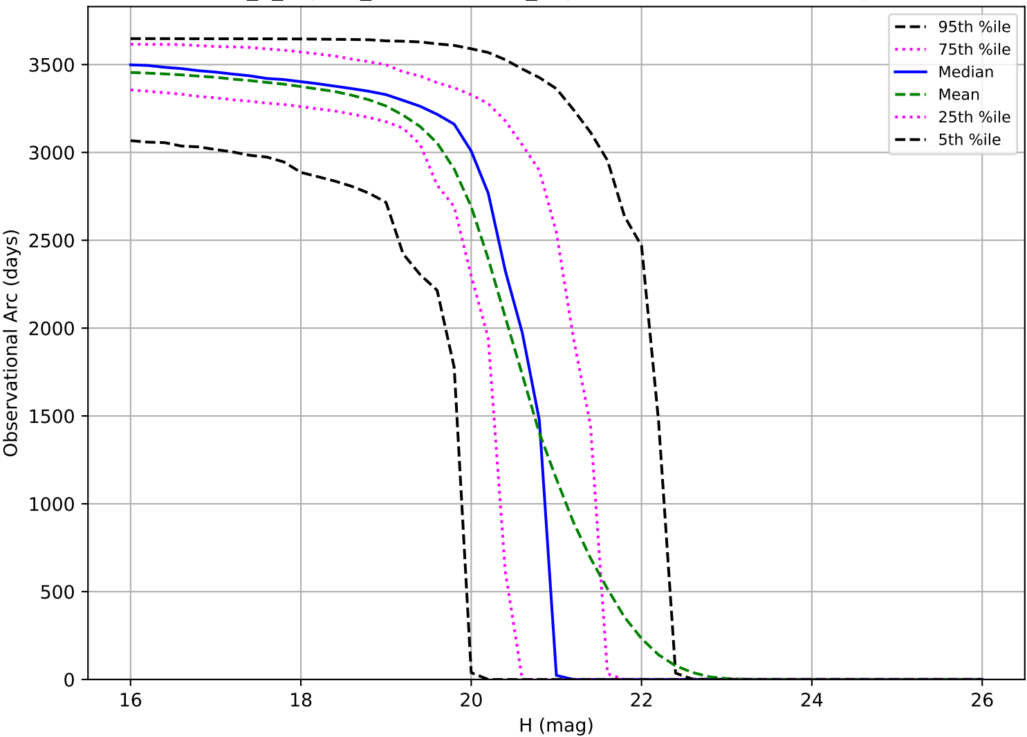
internal_u_expt30_nscale1.0v3.4_10yrs: Observational Arc Length MBA
