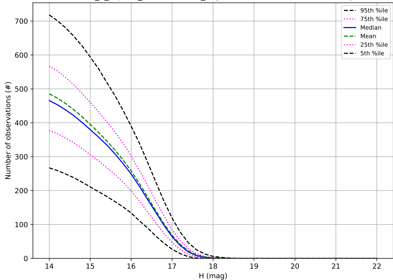
internal_u_expt30_nscale1.0v3.4_10yrs: Number of observations Trojan
