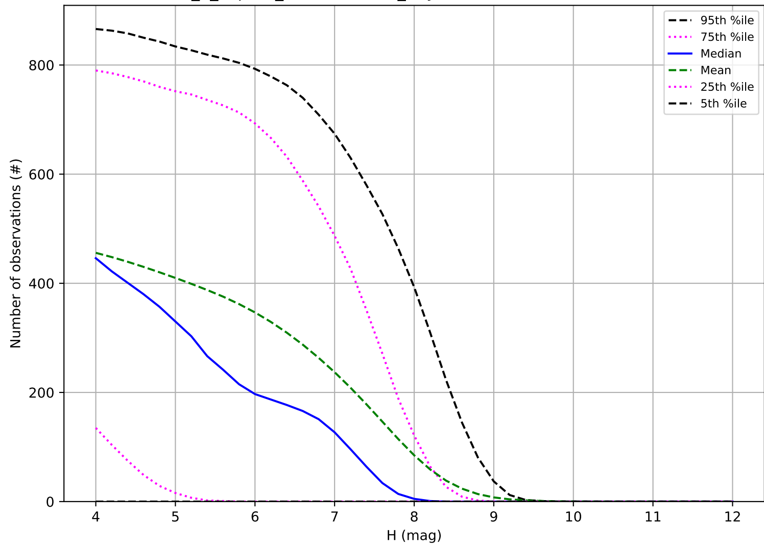
internal_u_expt30_nscale1.0v3.4_10yrs: Number of observations TNO
