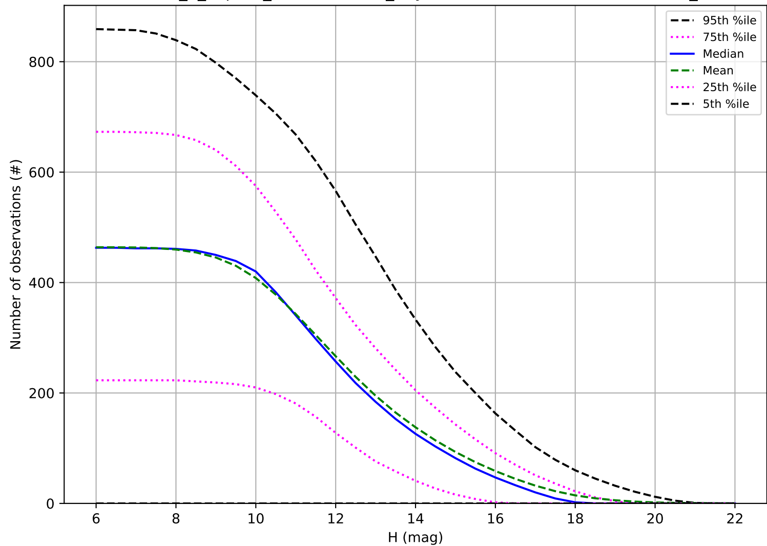
internal_u_expt30_nscale1.0v3.4_10yrs: Number of observations OCC_r5
