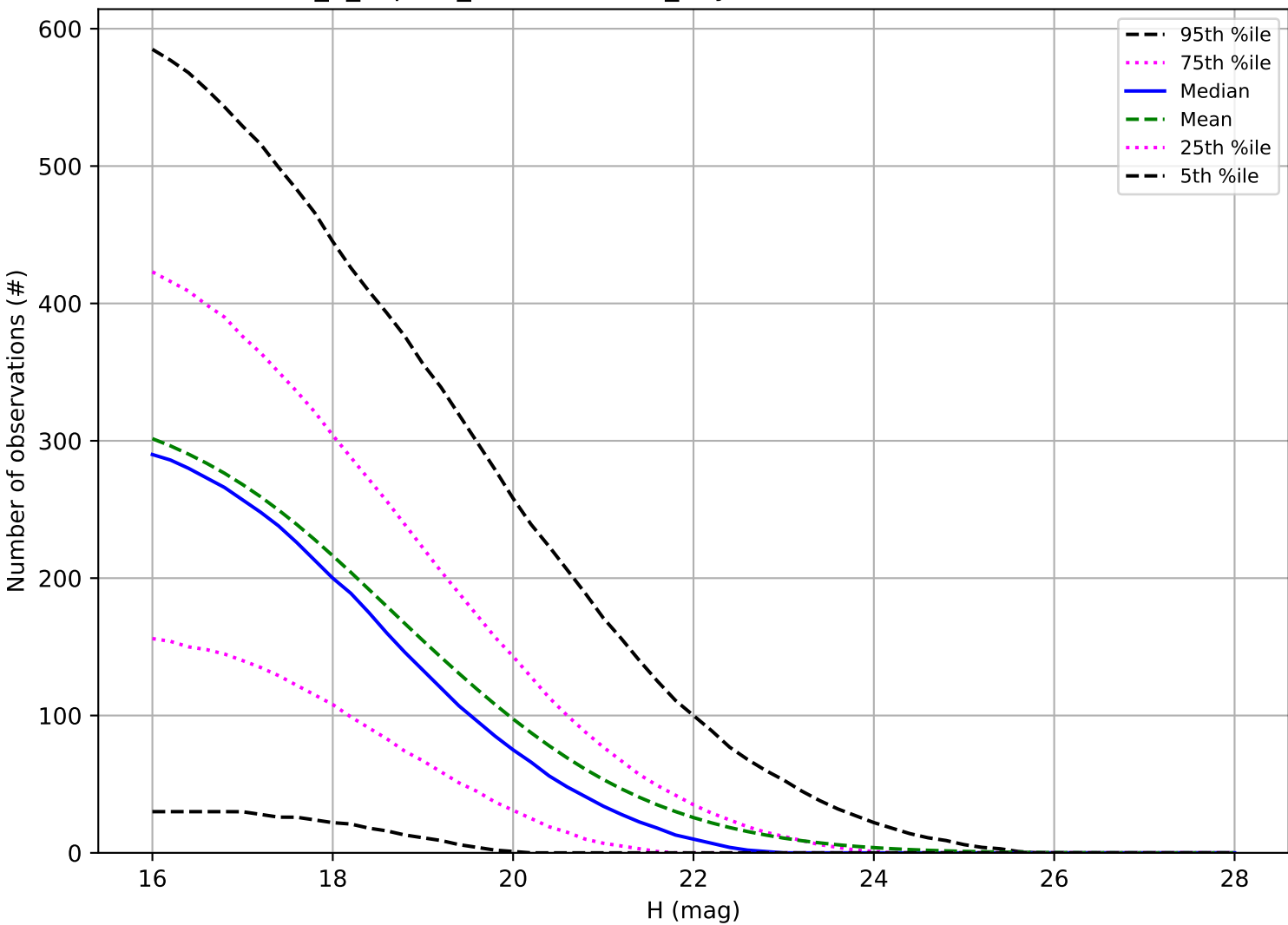
internal_u_expt30_nscale1.0v3.4_10yrs: Number of observations NEO
