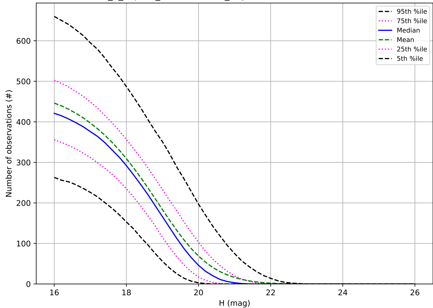
internal_u_expt30_nscale1.0v3.4_10yrs: Number of observations MBA
