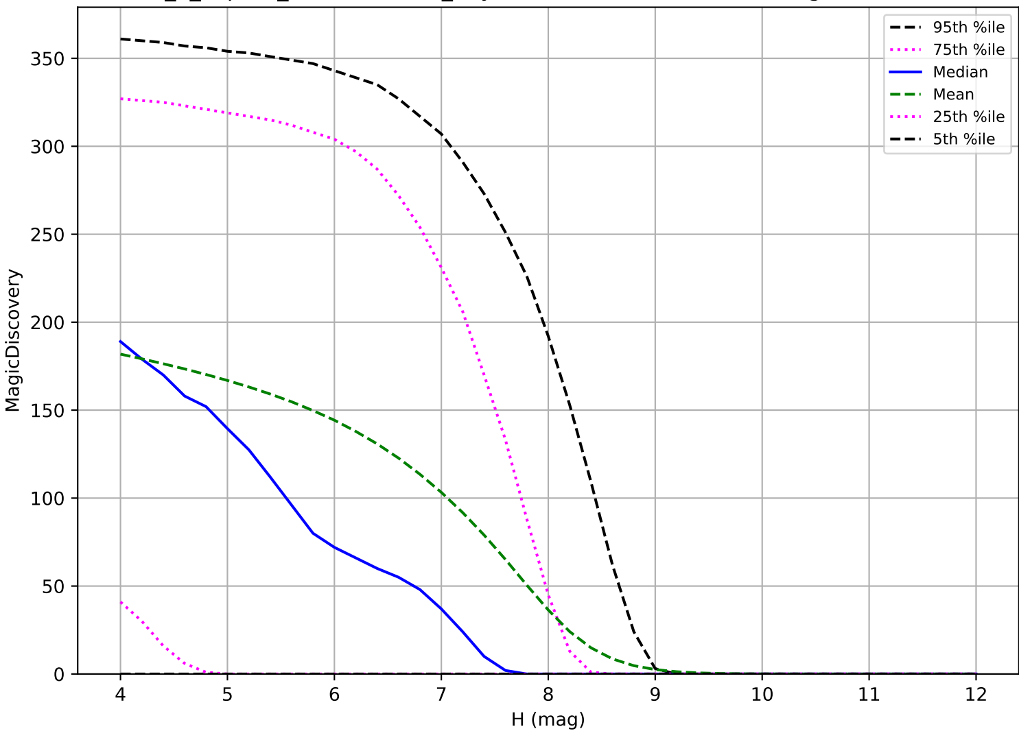
internal_u_expt30_nscale1.0v3.4_10yrs: TNO 6 detections in 60 nights detection loss
