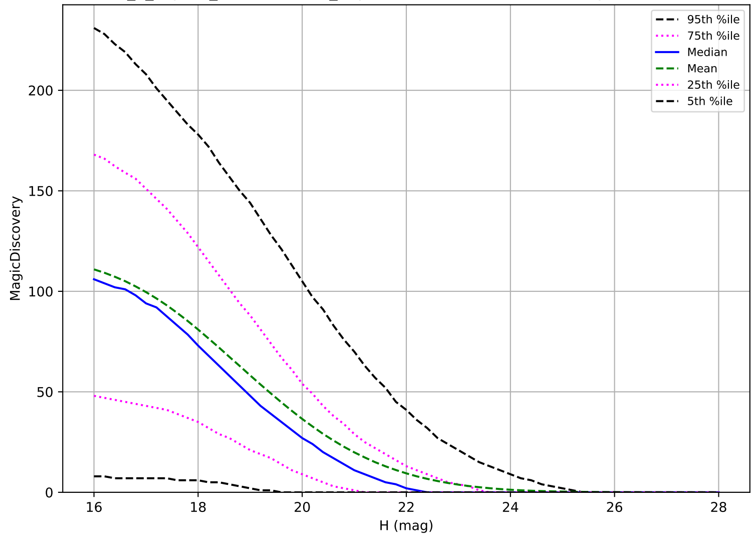
internal_u_expt30_nscale1.0v3.4_10yrs: PHA 6 detections in 60 nights detection loss
