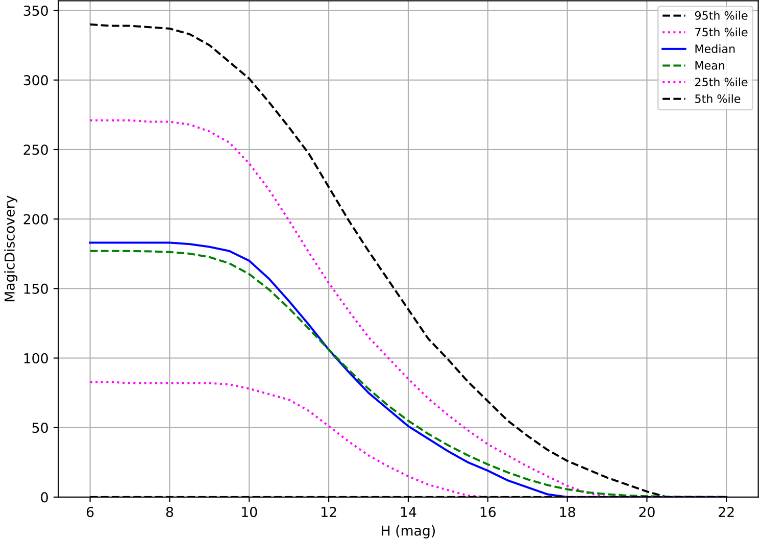
internal_u_expt30_nscale1.0v3.4_10yrs: OCC_r5 6 detections in 60 nights detection loss
