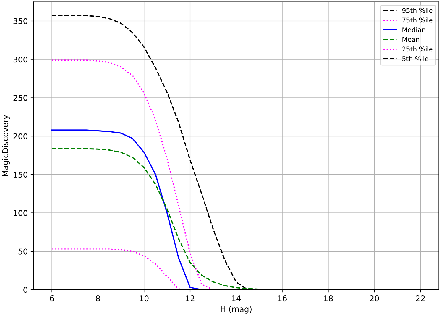
internal_u_expt30_nscale1.0v3.4_10yrs: OCC_r20 6 detections in 60 nights detection loss
