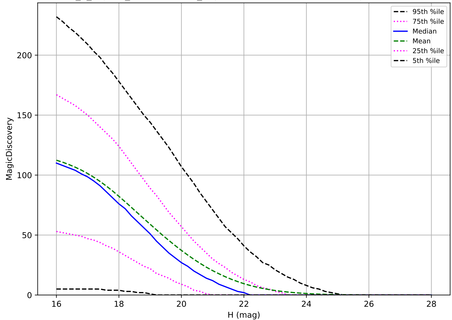
internal_u_expt30_nscale1.0v3.4_10yrs: NEO 6 detections in 60 nights detection loss
