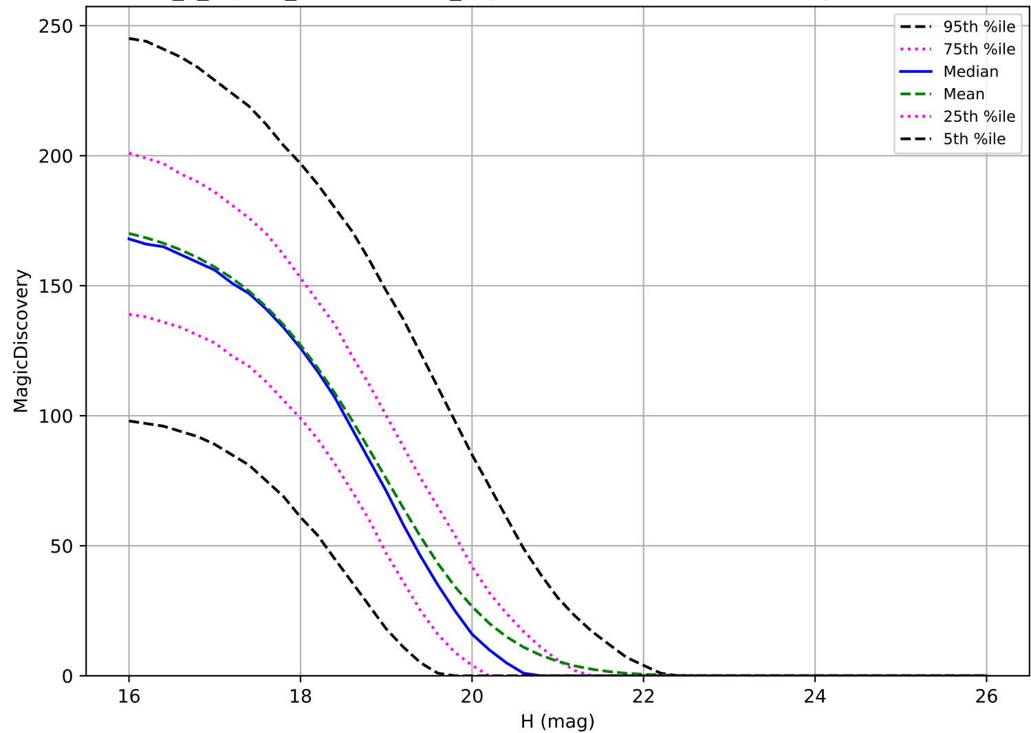
internal_u_expt30_nscale1.0v3.4_10yrs: MBA 6 detections in 60 nights detection loss
