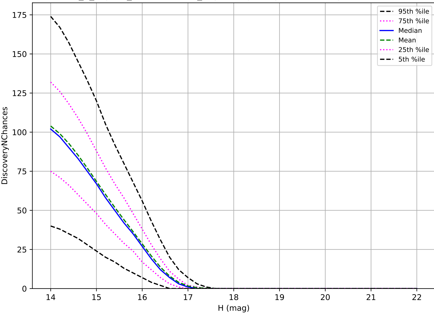
internal_u_expt30_nscale1.0v3.4_10yrs: Trojan 3 pairs in 15 nights detection loss
