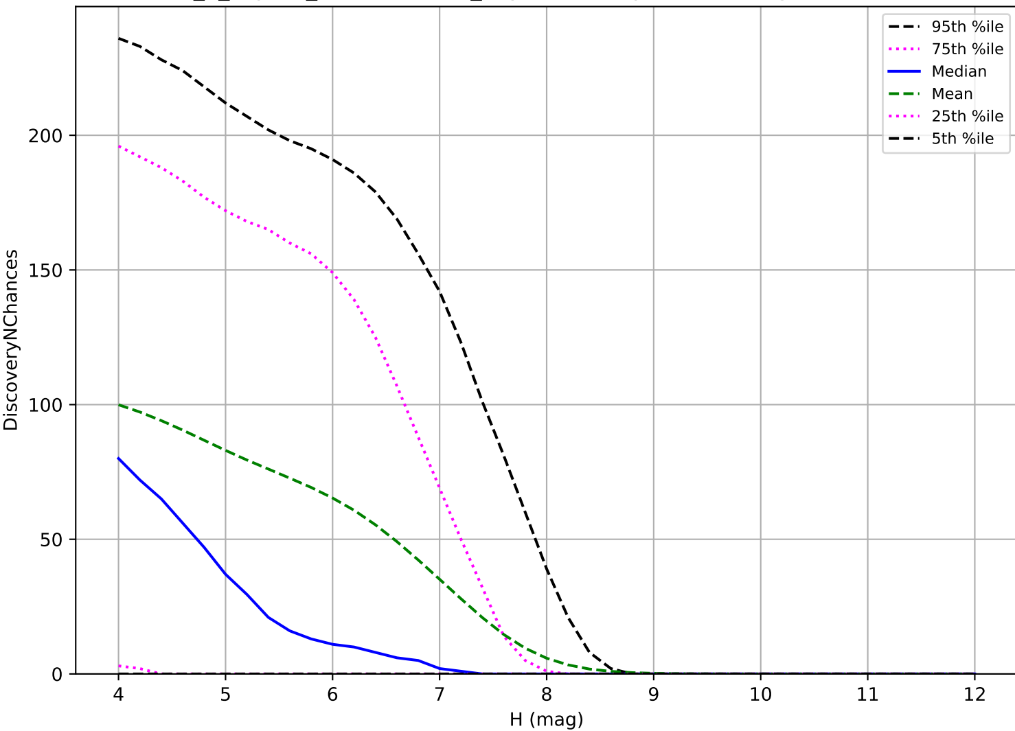
internal_u_expt30_nscale1.0v3.4_10yrs: TNO 3 pairs in 15 nights detection loss
