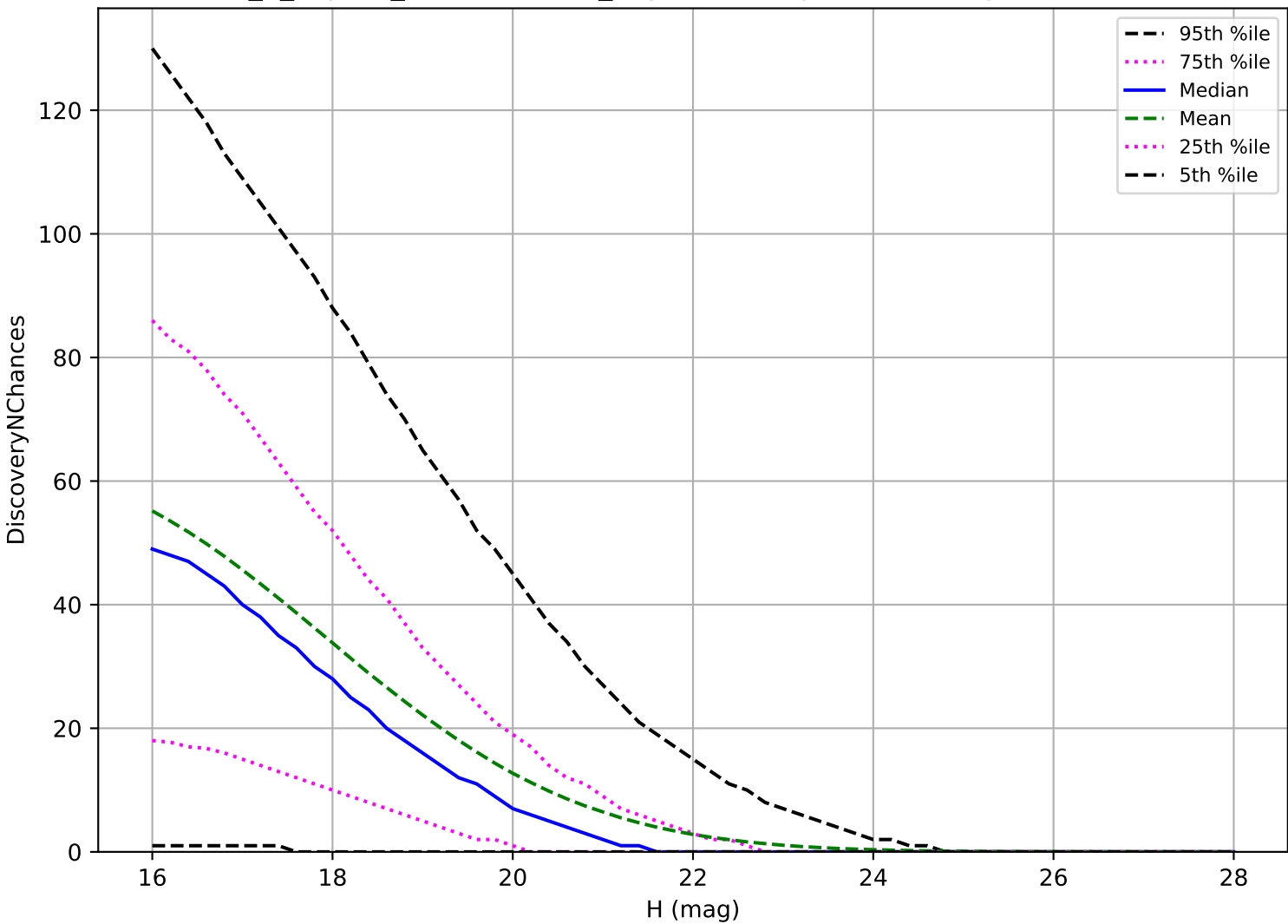
internal_u_expt30_nscale1.0v3.4_10yrs: PHA 3 pairs in 15 nights detection loss
