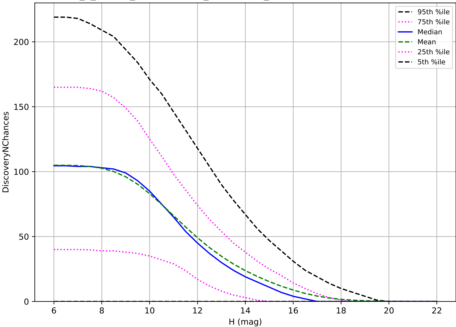
internal_u_expt30_nscale1.0v3.4_10yrs: OCC_r5 3 pairs in 15 nights detection loss
