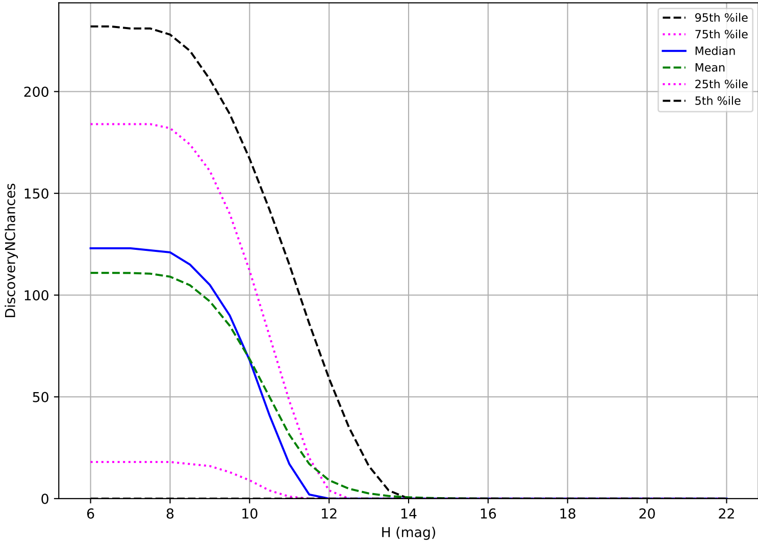
internal_u_expt30_nscale1.0v3.4_10yrs: OCC_r20 3 pairs in 15 nights detection loss
