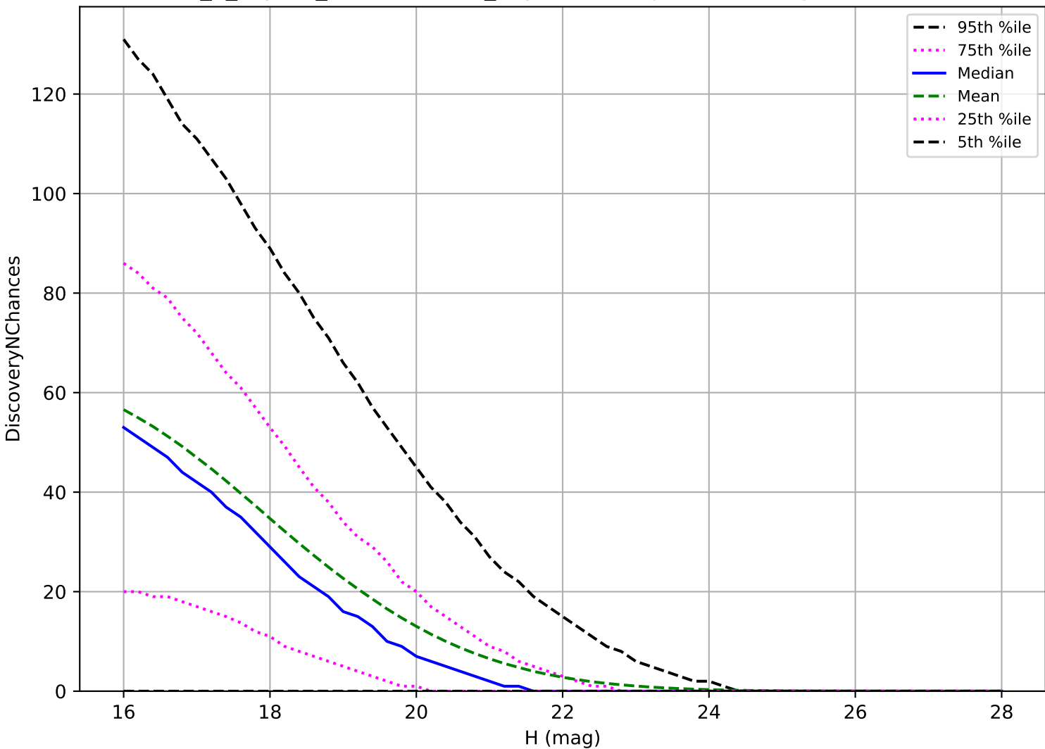
internal_u_expt30_nscale1.0v3.4_10yrs: NEO 3 pairs in 15 nights detection loss
