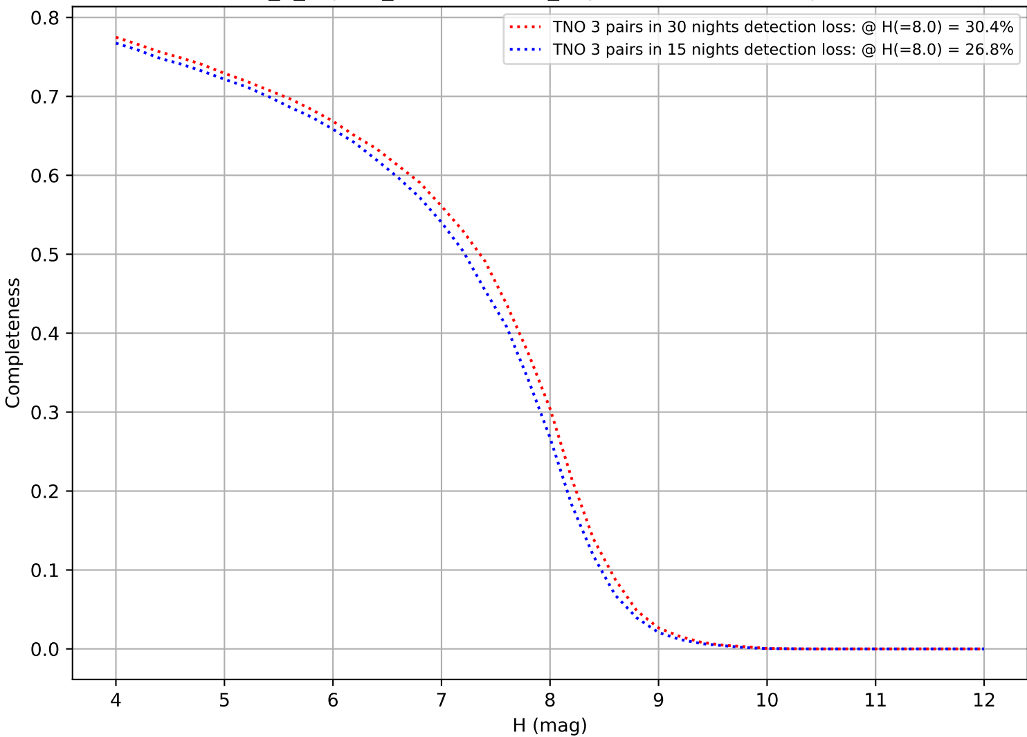
internal_u_expt30_nscale1.0v3.4_10yrs: DifferentialCompleteness
