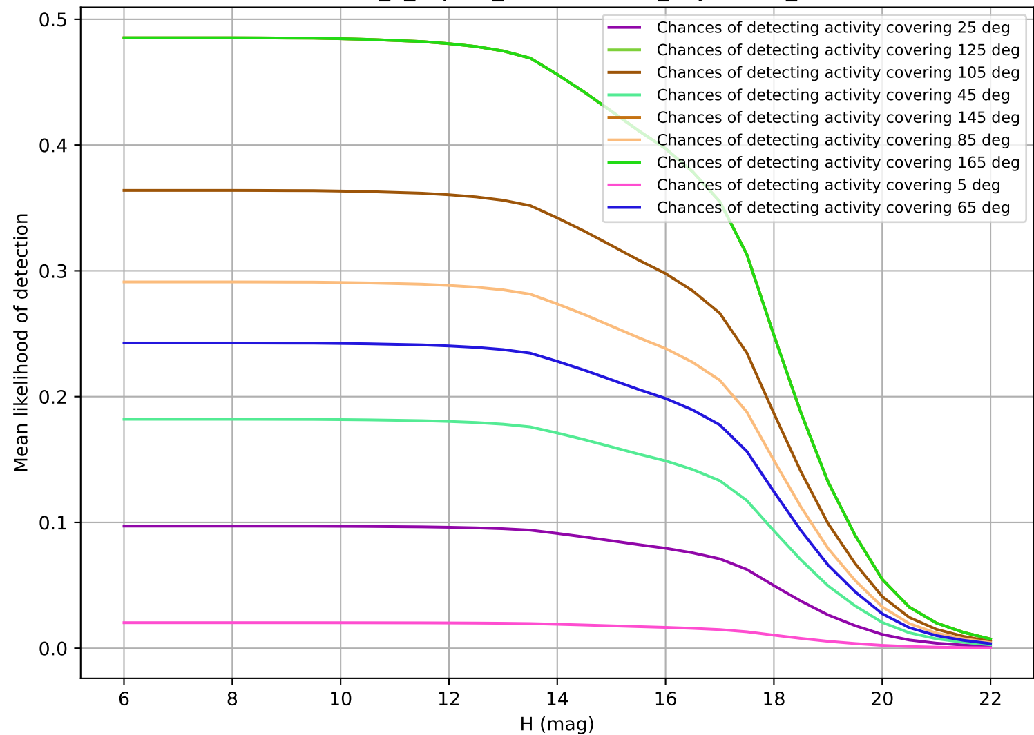
internal_u_expt30_nscale1.0v3.4_10yrs OCC_r5
