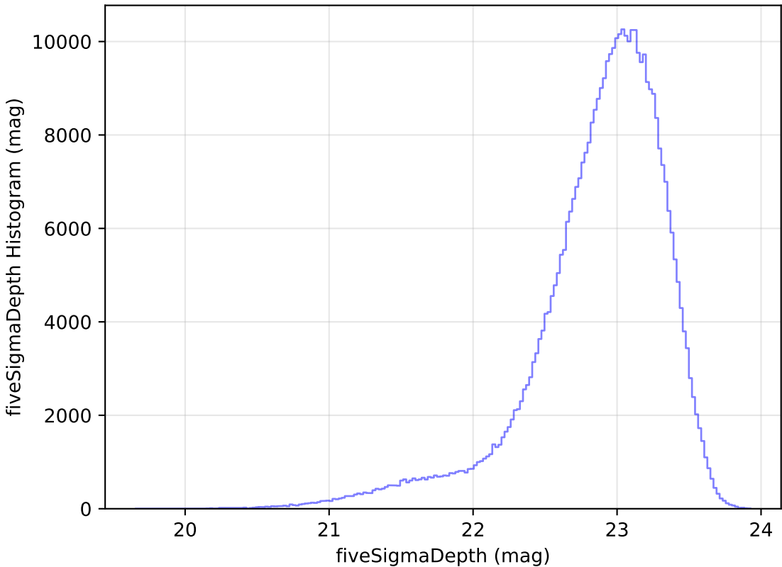
internal_u_expt30_nscale1.0v3.4_10yrs z: fiveSigmaDepth Histogram
